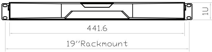
Front View
